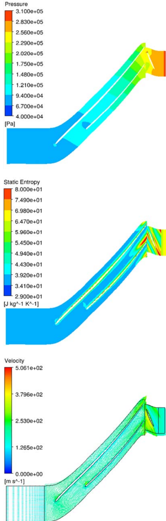
Figure 9. 50% blade height position pressure, entropy, velocity distribution.
